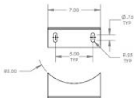
Detail MOUNTING BRACKET (x2)
